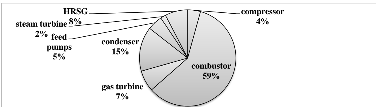
Figure 4. Exergy destruction distribution in CCPP.
