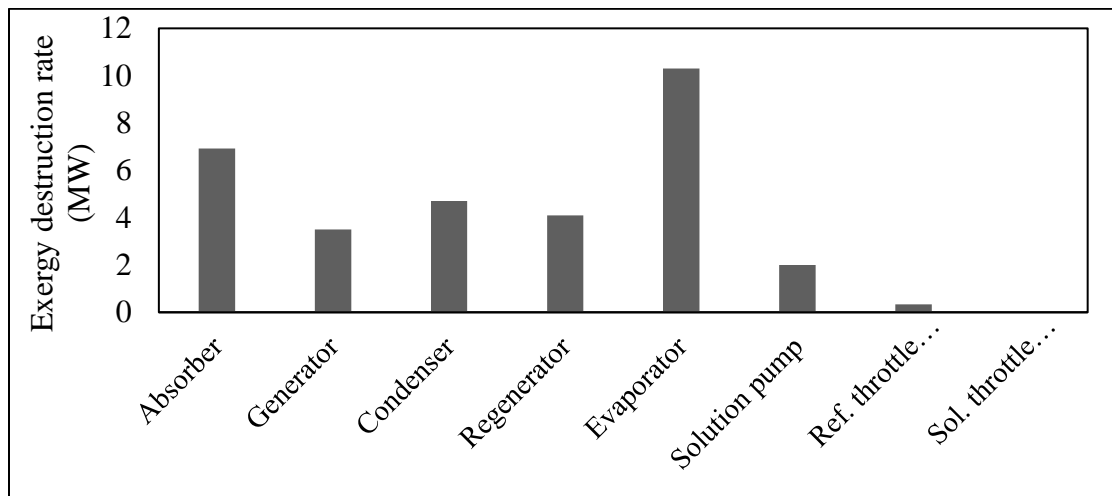
Figure 5. Rates of exergy destruction distribution in the absorption refrigeration system.
