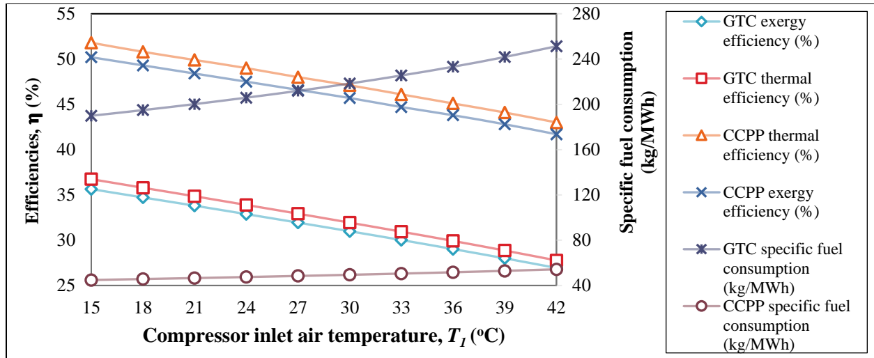
Figure 8. Variations of the gas turbine cycle and combined cycle power plant efficiencies, and specific fuel consumption, SFC (kg/MWh), with ambient inlet air temperature, T_l .
