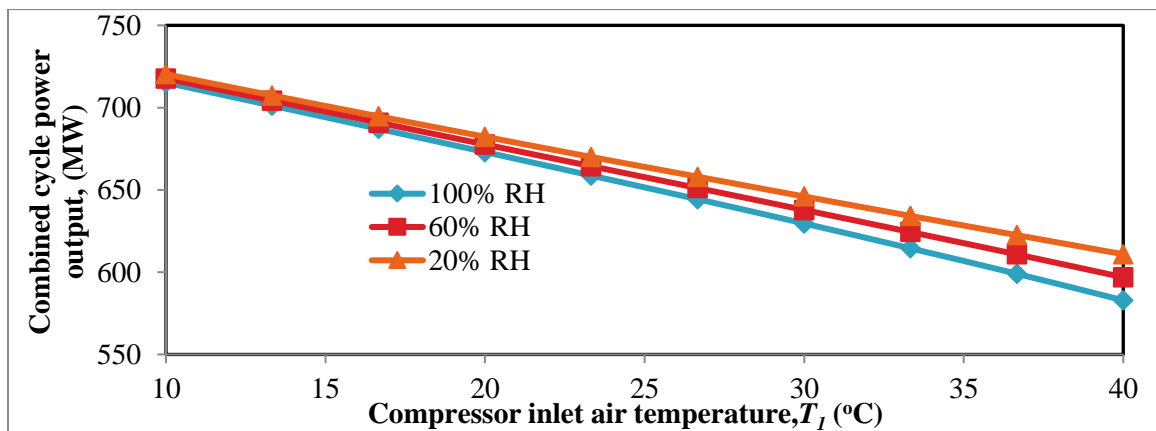
Figure 7. Effects of varying ambient temperature and relative humidity on the CCPP power output.
