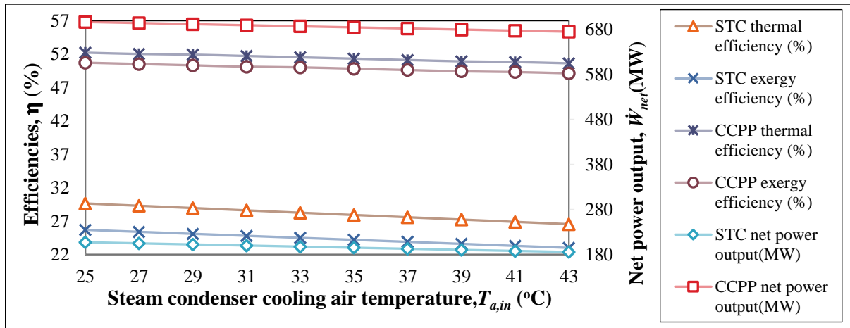
Figure 9. Steam condenser cooling air temperature versus steam turbine, combined cycle plant power output, energy and exergy efficiencies.
